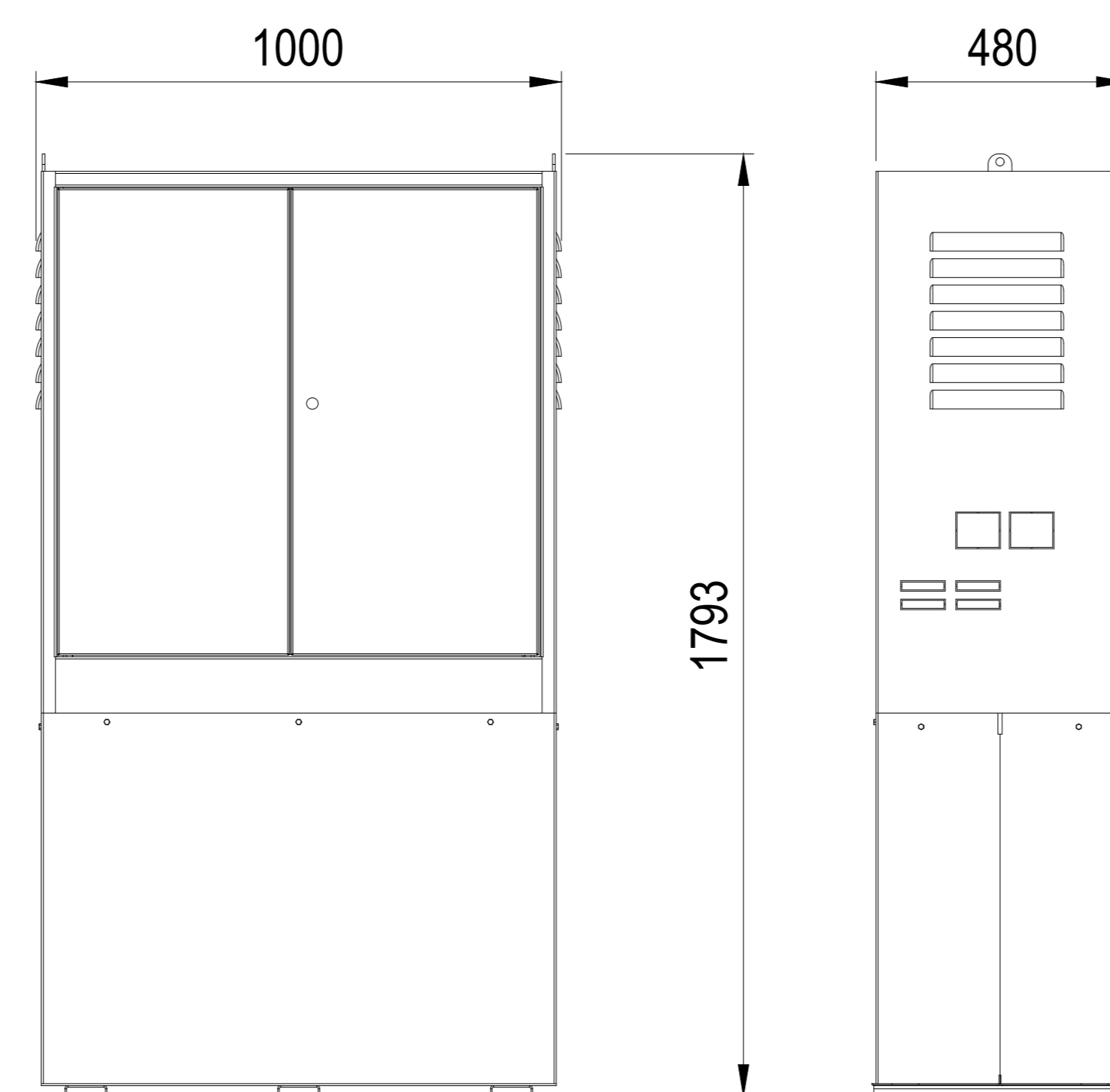
Lift Machinery Cabinet with integrated hydraulic tank. Must be located within 8m of lift well
